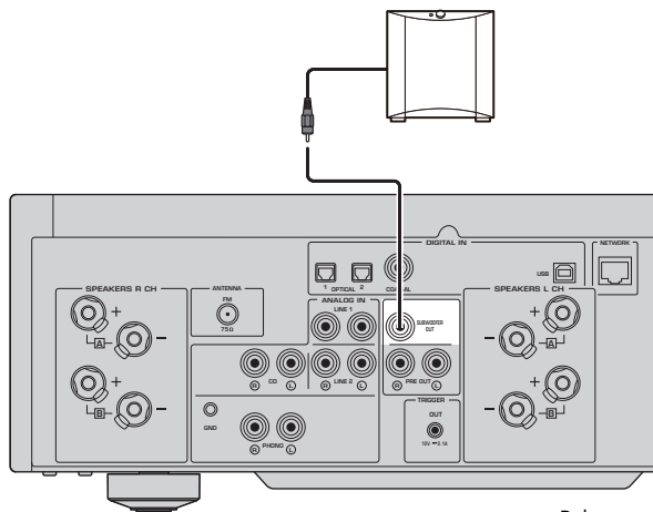
Bakre panel
