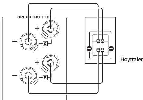
Bakre panel
